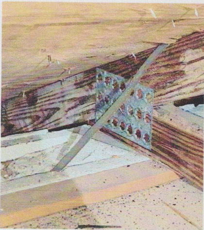
Toe Nailed (Metal connectors that do not meet the minimum requirements)
